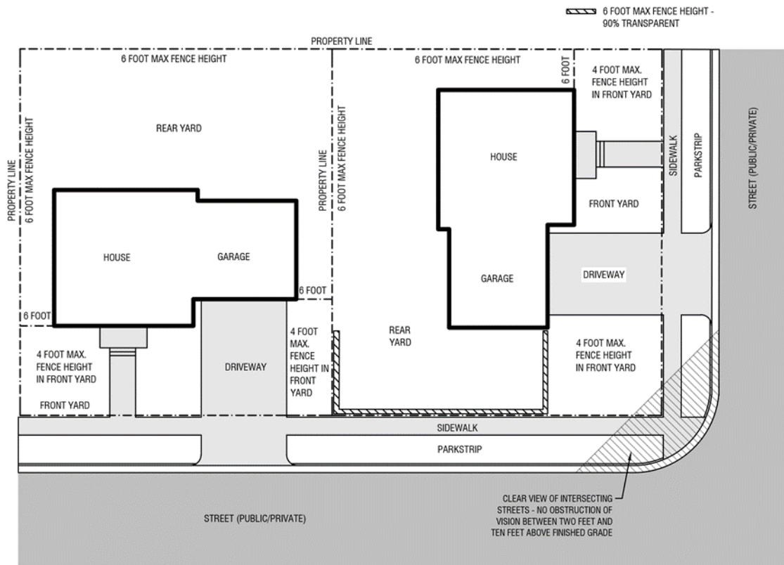
Figure 10-12-2 Corner Lot Fencing Requirements
